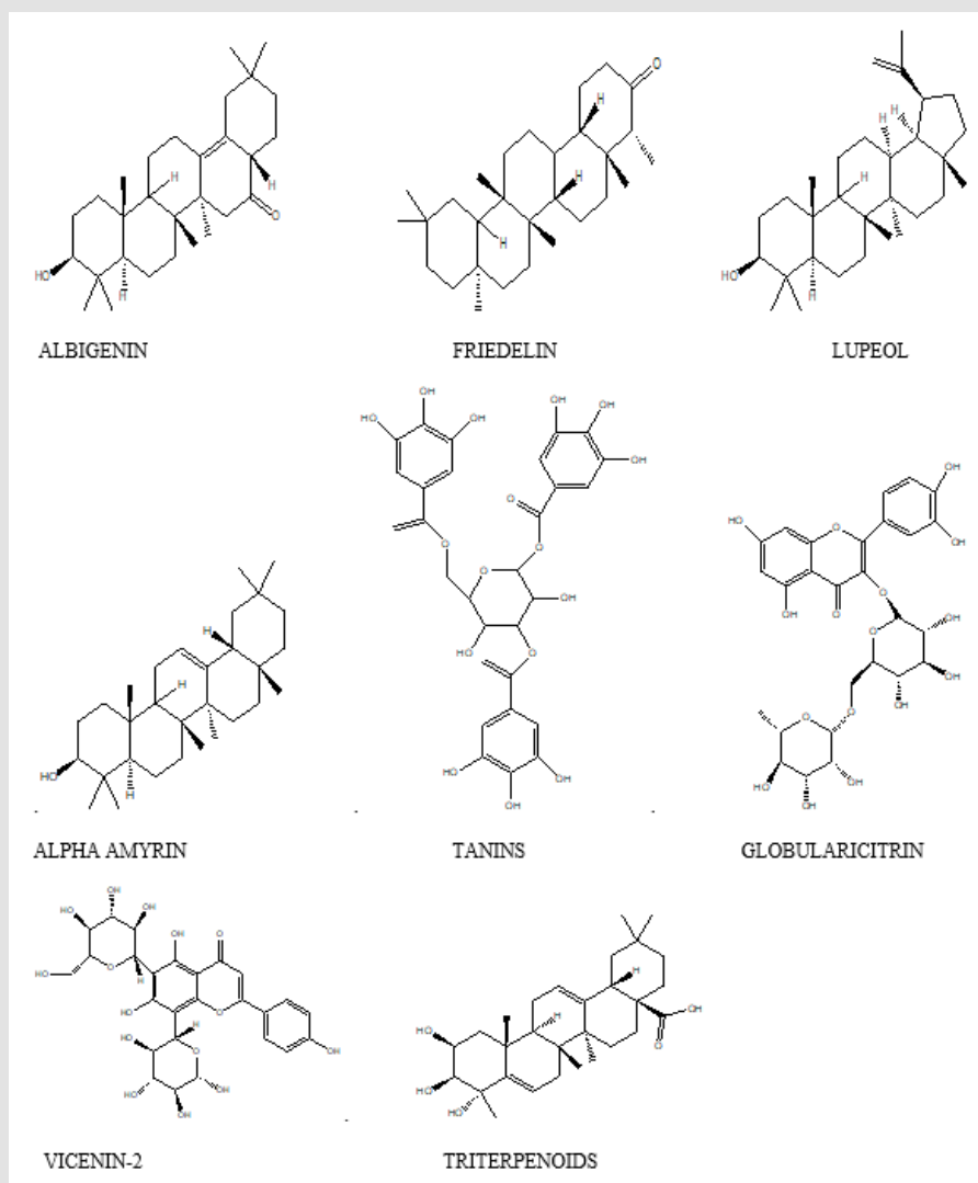
Figure 2: Phytoconstituents of Albizia lebeck with highest binding energy with receptors of ARDS.
