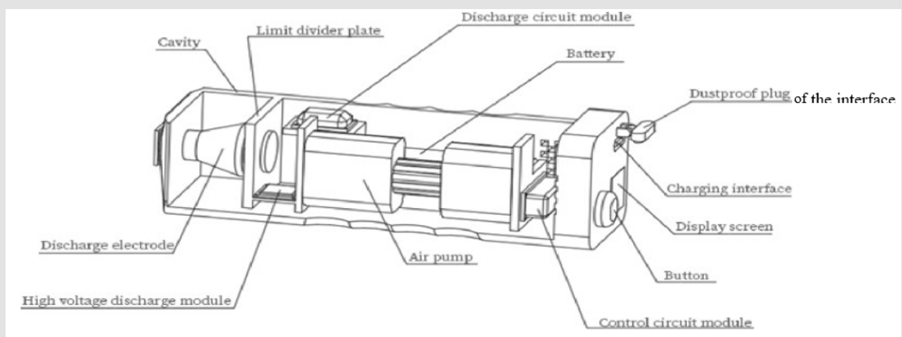
Figure 3: Schematic diagram of the structure of a portable low – temperature air plasma jet coagulation device.
